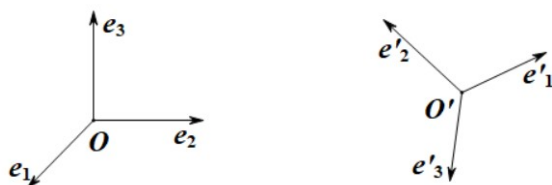
图 3.15: 坐标变换 \{O; \mathbf{e}_1, \mathbf{e}_2, \mathbf{e}_3\} \xrightarrow{\phi} \{O'; \mathbf{e}'_1, \mathbf{e}'_2, \mathbf{e}'_3\}
